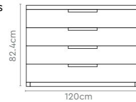
Chest of Drawers (1200mm)
