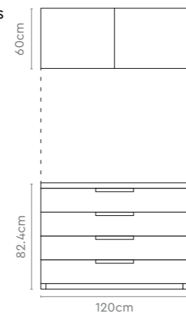
Chest of Drawers (1200mm) + OHU*
